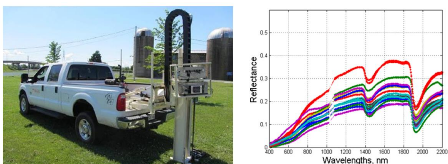
Figure 6 Optical sensor with visible and near-infrared spectrum (left) and soil spectra obtained from the optical sensor (right) 30
